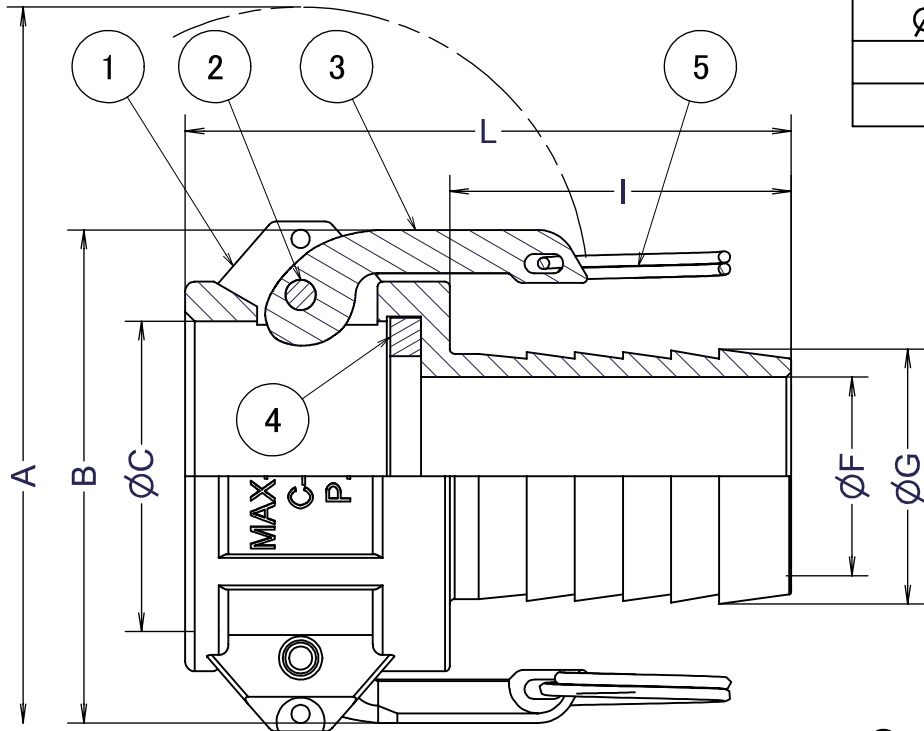
Section C-C
