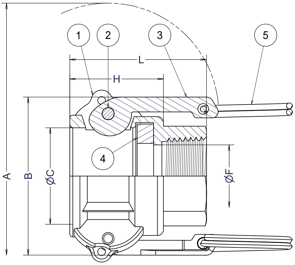
Section C-C
