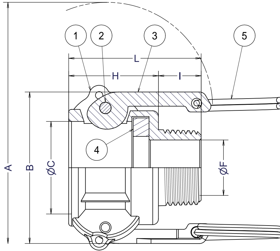
Section C-C
