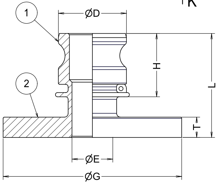
Section K-K
